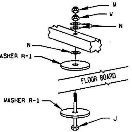
Figure 1.2 OPTIOAL Example configuration using R-1 Washers
